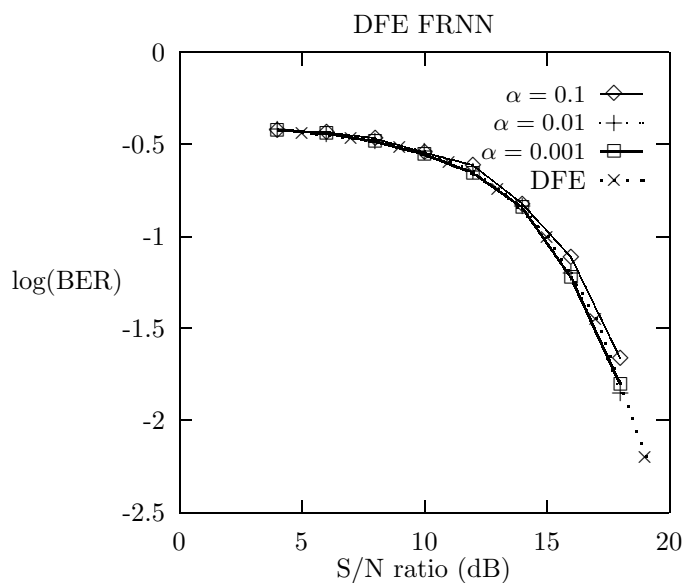
Figure 3. Bit error rate versus signal-noise ratio for the FRNN emulating the optimum DFE for the channel, before and after training.
