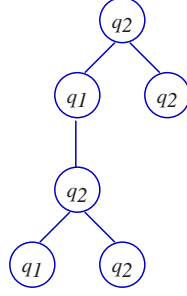
Fig. 2: Output states after the computation of the tree automaton A on a(a(a(ab))b) .
