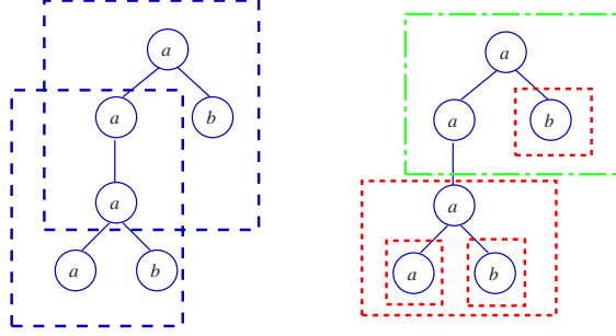
Fig. 3: Left: set of 3-forks contained in a(a(a(ab))b) . Right: 2-root (dash-dotted) and 2-subtrees.
