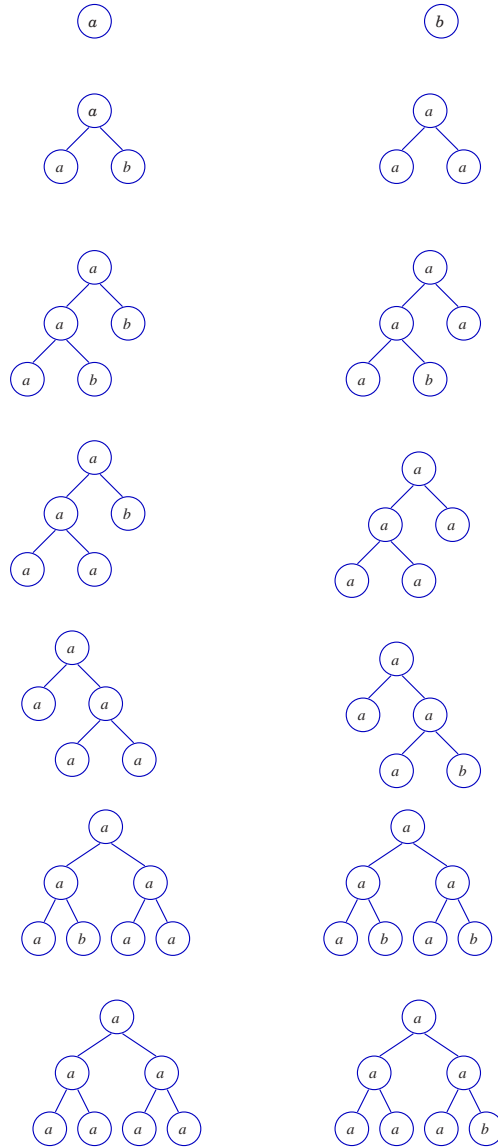
Fig. 4: Set \Theta^{[3]} of 2-subtrees and 3-forks generated by the automaton A with the transitions defined in eq. (16).
