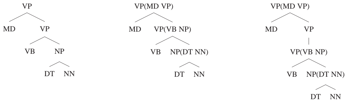
Fig. 6: Parse tree obtained with G^{[2]} (left); parse tree obtained with G^{[3]} , invalid if the rule VP(MD VP) \rightarrow MD VP(VB NP) is missing in R^{[3]} (middle); parse tree obtained with G' where backoff rules VP(MD VP) \rightarrow MD VP and VP \rightarrow VP(VB NP) have been applied (right).
